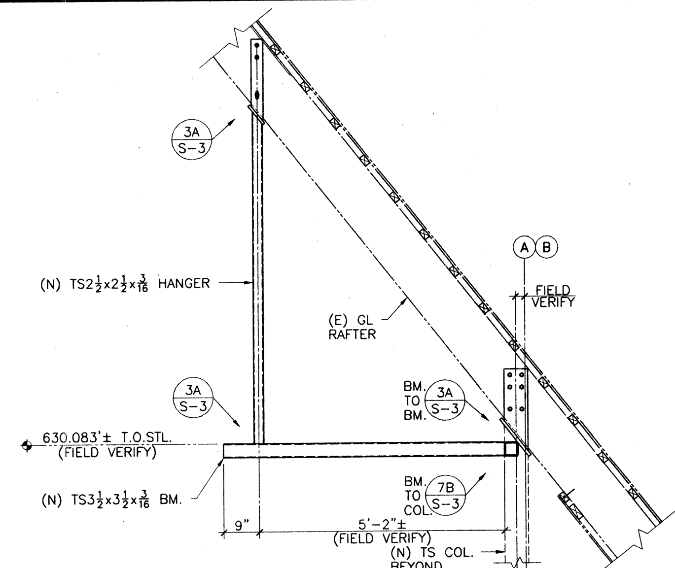
HAMMERBEAM AT SANCTUARY
