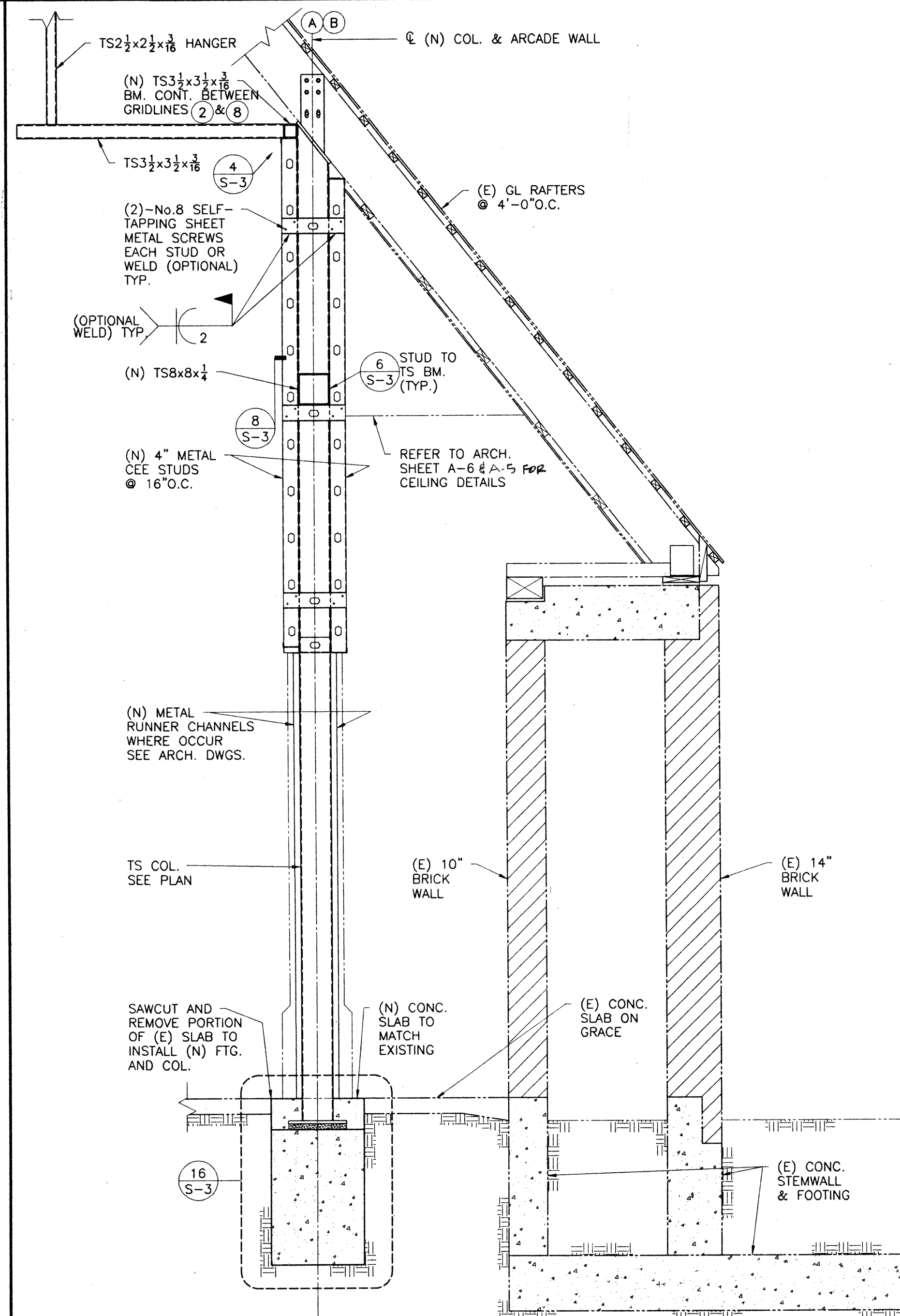
TYPICAL ARCADE WALL SECTION AT COLUMN
