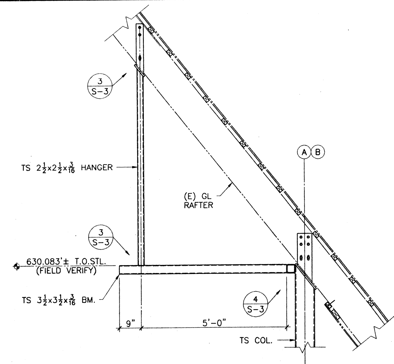
TYPICAL HAMMERBEAM AT NAVE
