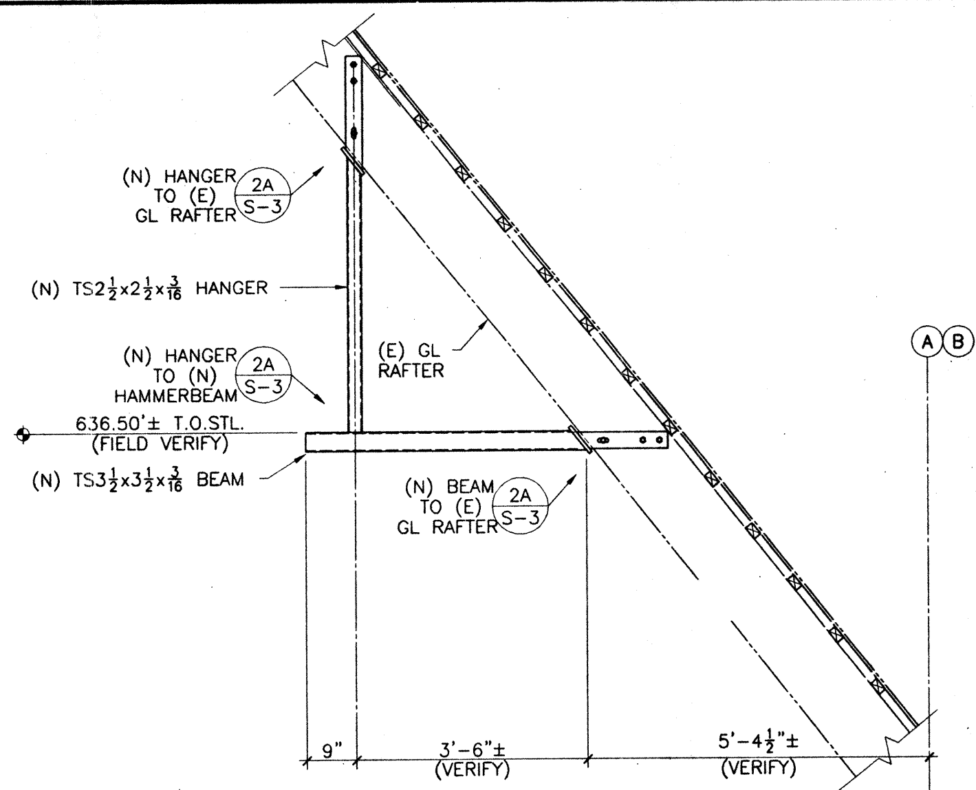
HAMMERBEAM AT SANCTUARY
