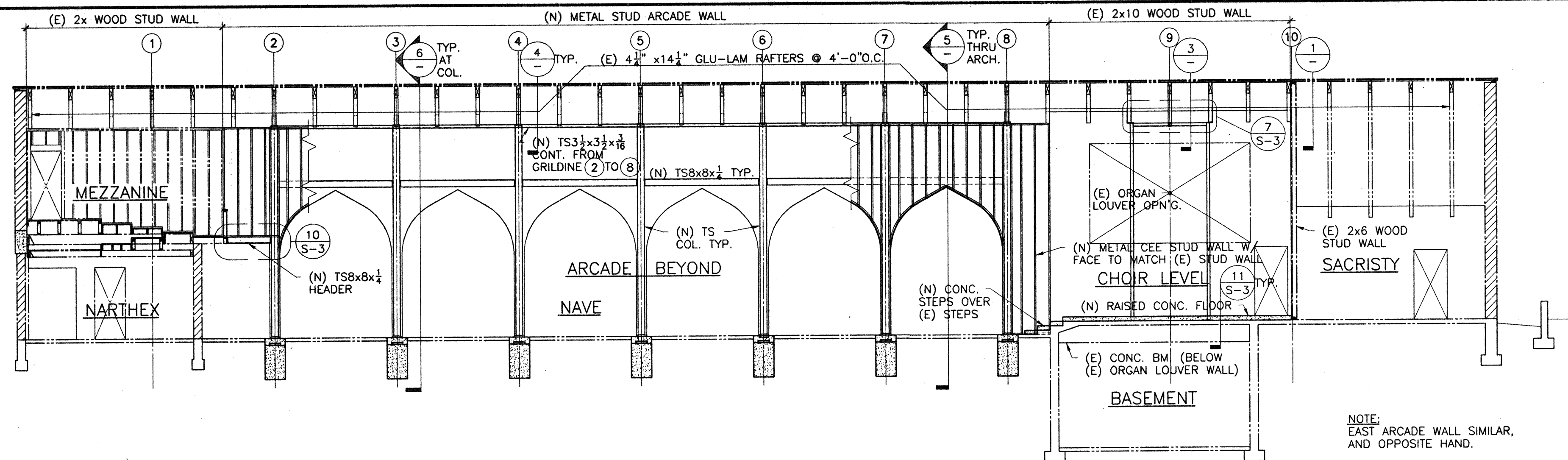
NEW INTERIOR WEST ARCADE WALL ELEVATION (LOOKING WEST)
