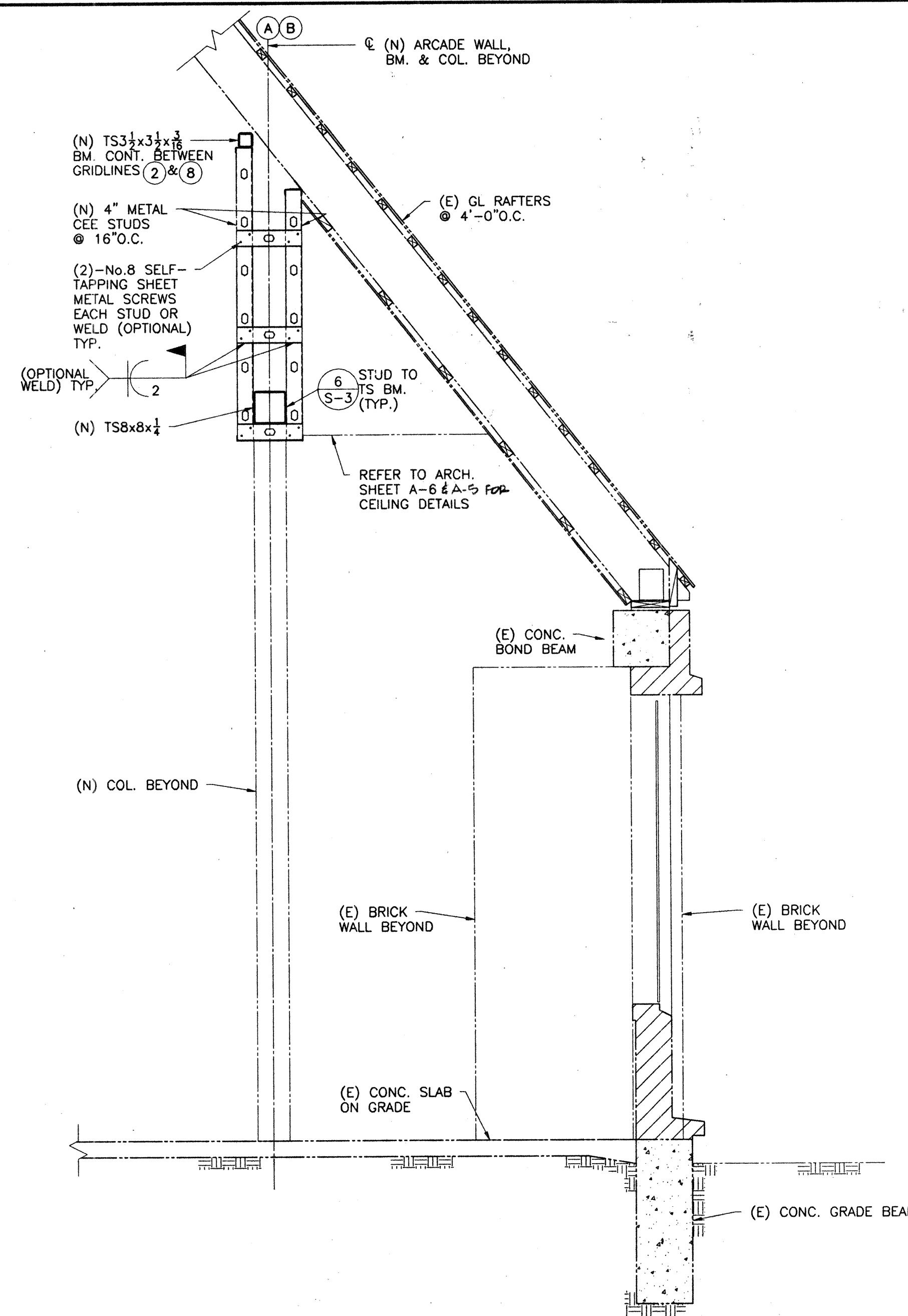
NEW INTERIOR WEST ARCADE WALL ELEVATION (LOOKING WEST)
